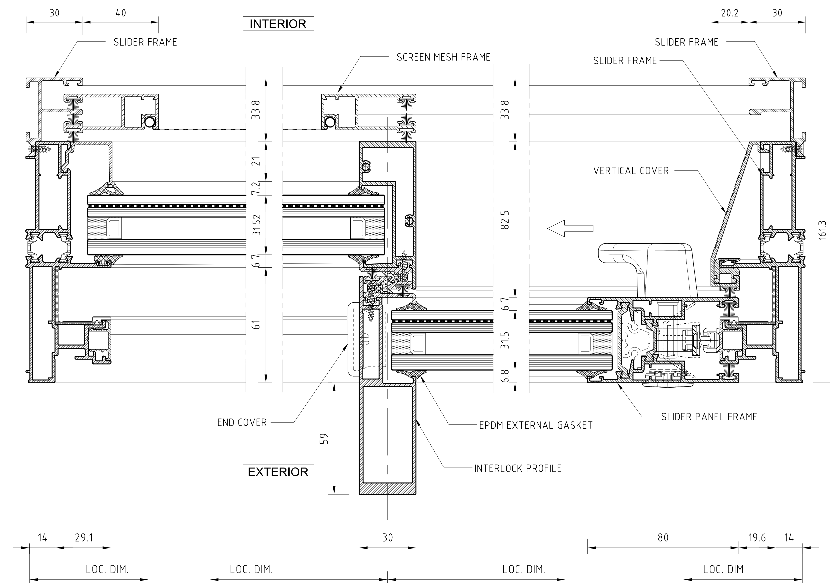
JAMB DETAIL FIXED SIDE
